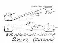
Figs. 1294-1295. Brake-shaft Stirrup Braces (2 of each).
